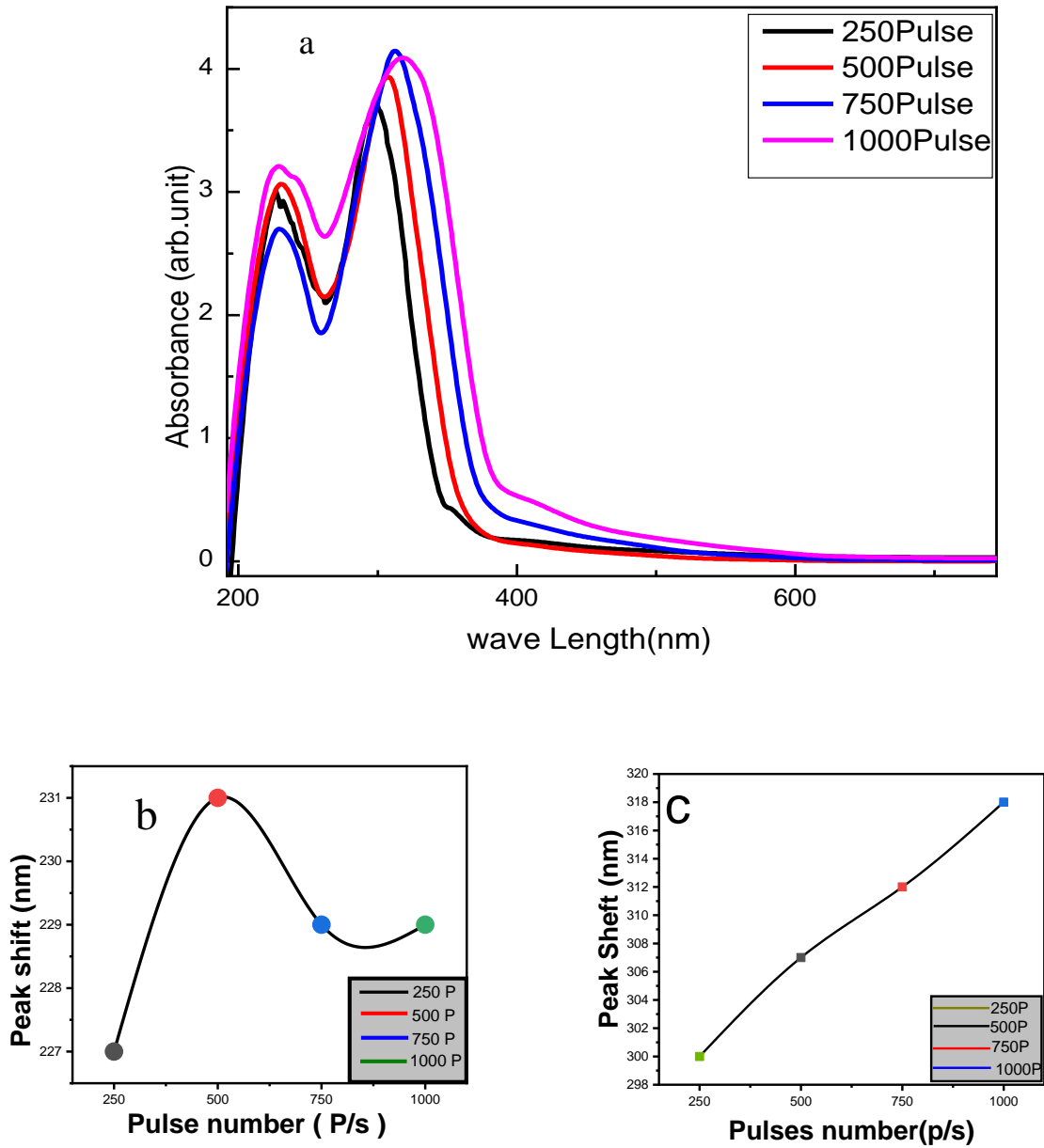
Fig.3: (a) CNP optical absorption spectrum prepared in an ethanol medium with multiple laser pulses (b) peak (minor) shift (c) peak (prominent) shift.
