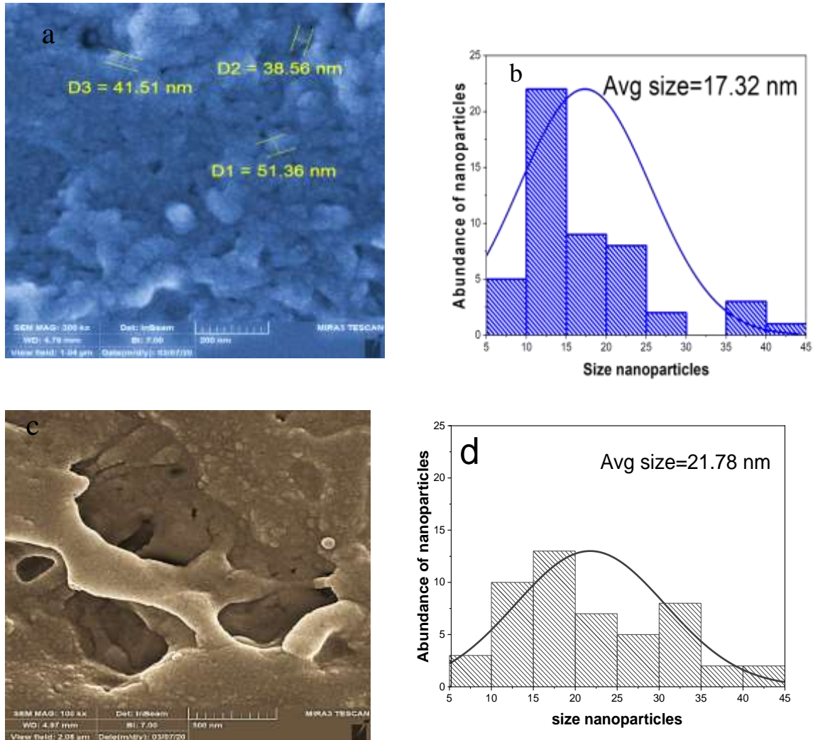
Fig. 2 : CNPs synthesized with optimum pulses laser in ethanol (a) FESEM image of the synthesized sample at (1000)Pulse / sec (b) Distribution of the scale of CNPs relating to (a), (c) FESEM image of the optimum sample at (500)Pulse/sec (d) Distribution of the scale of CNPs relating to (c).
