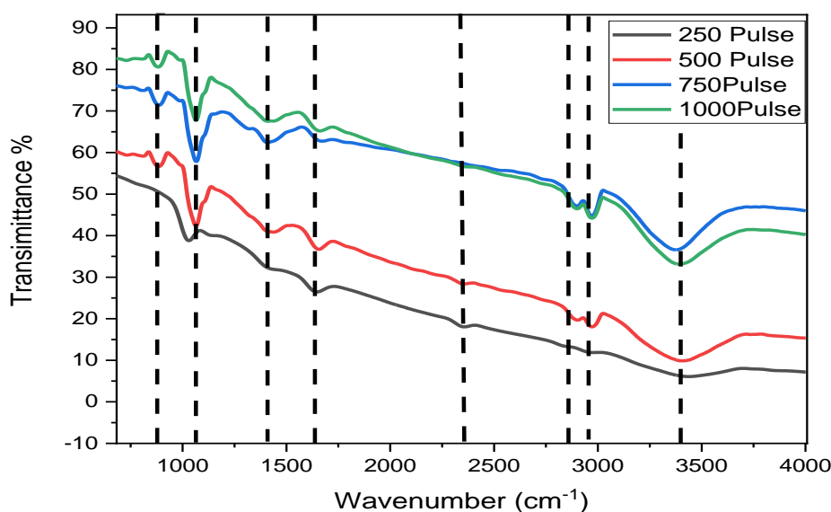
Fig. 4: FTIR spectrum, depending on the change in the number of pulses.
