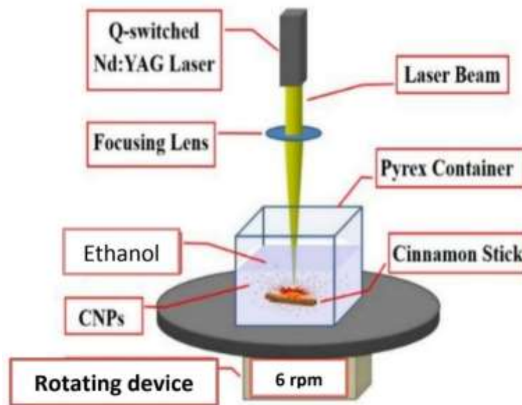
Fig 1: Schematic diagram of the "pulsed laser ablation in Liquid system" (PLAL).
