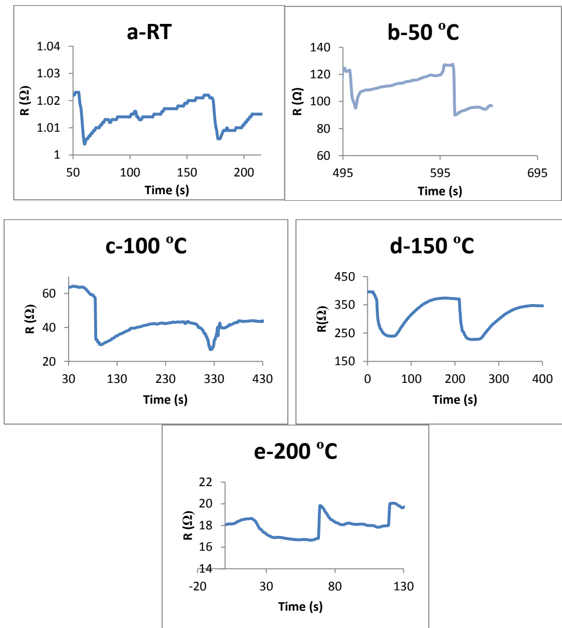
Fig.4: Resistance-time variation of F-MWCNTs sensor time at a-RT, b-50 c-100 d-150 and e-200 testing temperature upon exposure to NO_2 gas.
