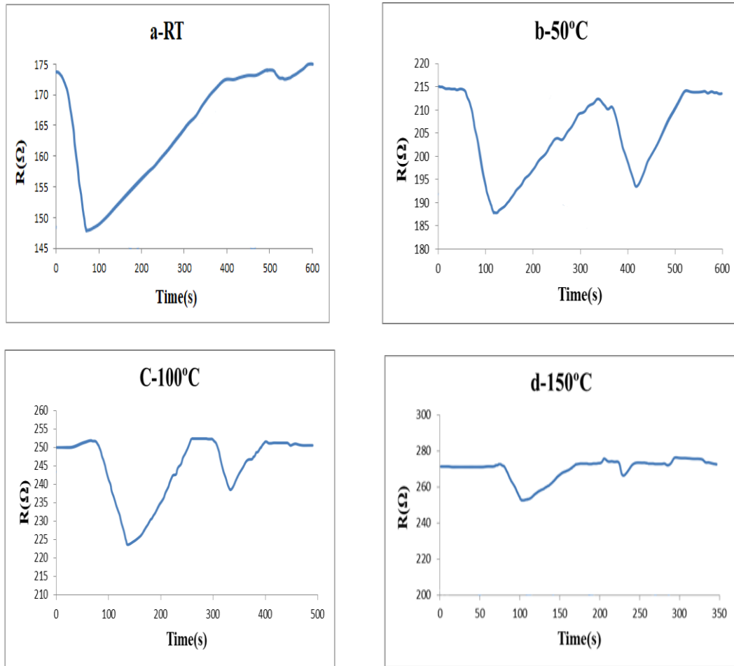
Fig.6: Resistance-Time curves of FSWCNTs/CoO NPs sensor at RT, 50 °C, 100 °C, 150 °C when exposed to NO 2 gas.
