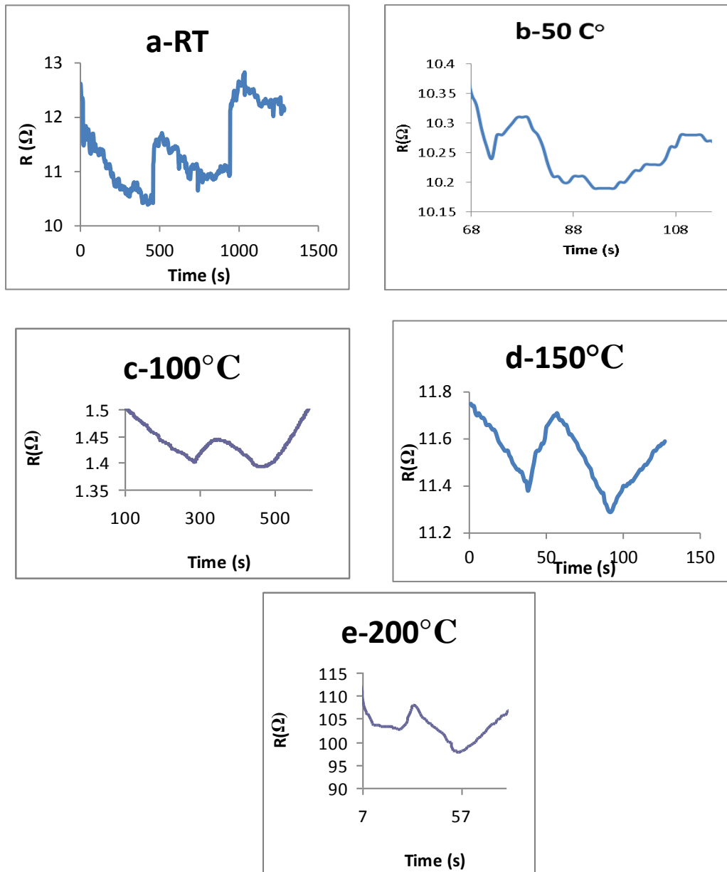
Fig.3: Resistance-time variation of F-SWCNTs sensor time at a-RT, b-50 c-100 d-150 and e-200 testing temperature upon exposure to NO 2 gas.
