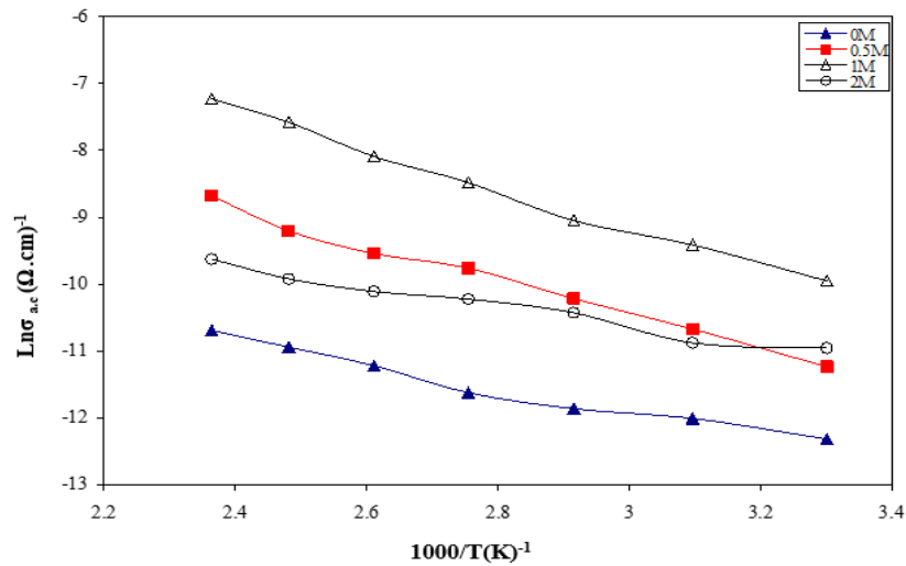
Figure 7: Temperature dependence of \ln(\sigma_{a.c}) for pure PANI and doped with H_2SO_4 at 10 KHz.
