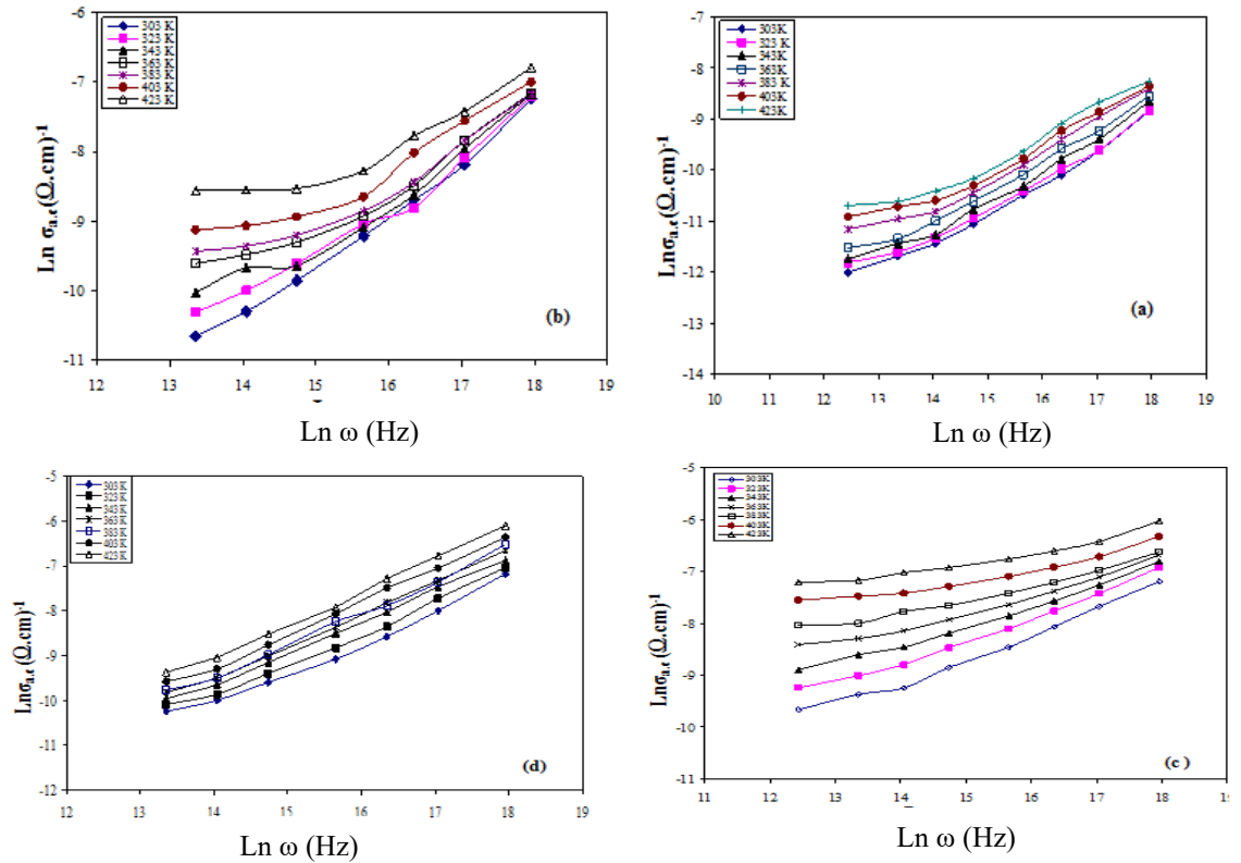
Figure 5: \ln \sigma_{ac} as a function of \ln \omega for (a) pure PANI, (b) 0.5 M, (c) 1M, and (d) 2M H_2SO_4 doping at different temperatures
