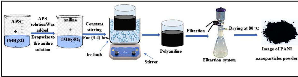
Figure 1: The preparation process of PAN.
