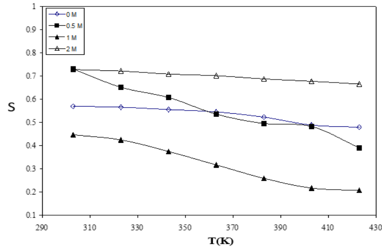
Figure 6: Exponential factor ( s ) as a function of temperature.
