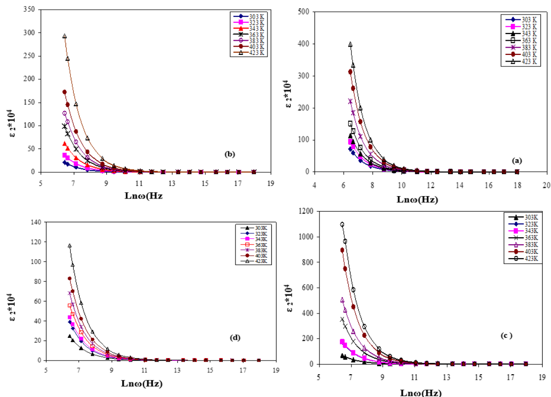
Figure.10: Frequency dependence of dielectric losses for (a) polyaniline pure, (b) 0.5 M, (c) 1M, and (d) 2M H 2 SO 4 doping at different temperatures.
