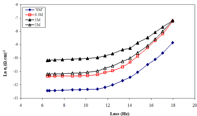
Figure: 8 Frequency dependence of conductivity for different \text{H}_2\text{SO}_4 molarity.
