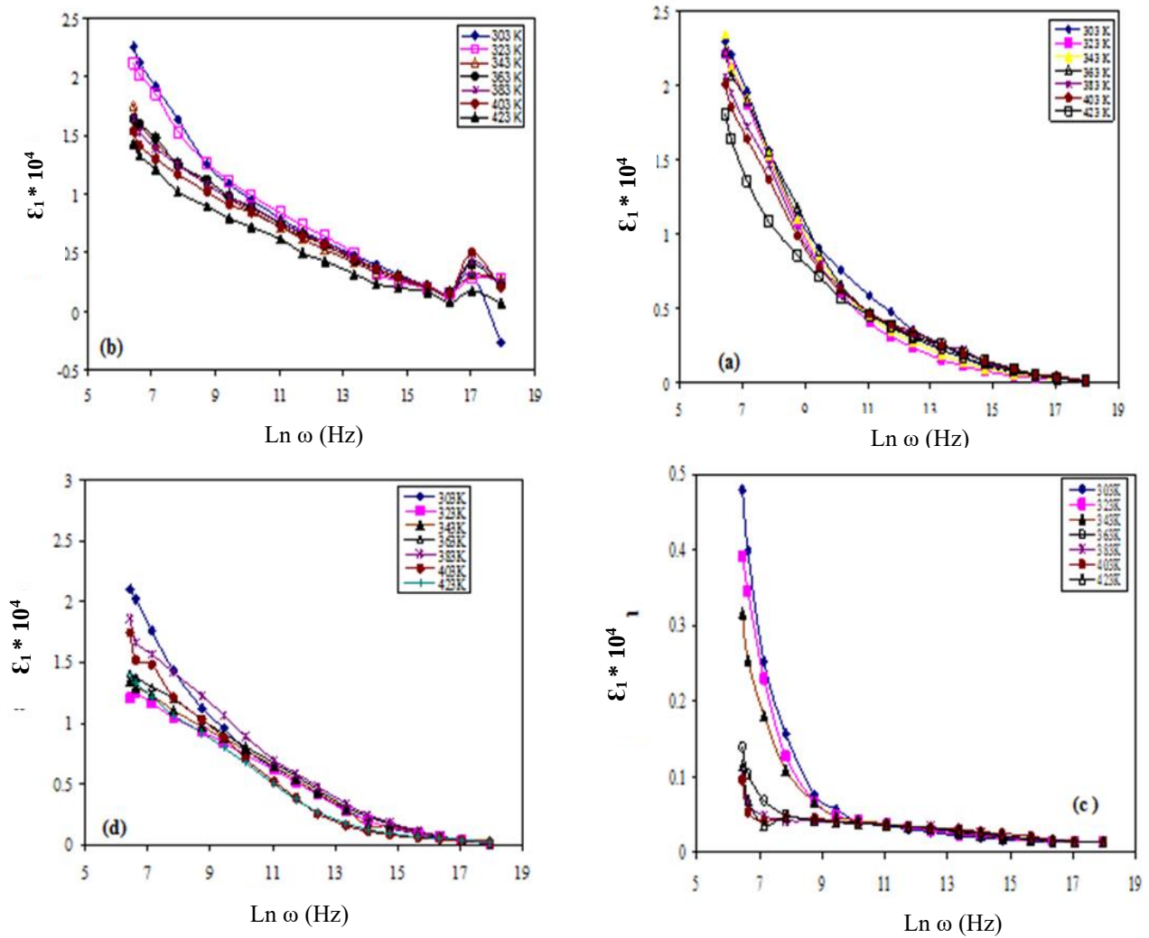
Figure 9: The real part of the dielectric constant dependence on \ln \omega for: (a) pure PANI, (b) 0.5 M, (c) 1M, and (d) 2M H_2SO_4 doping at different temperatures.
