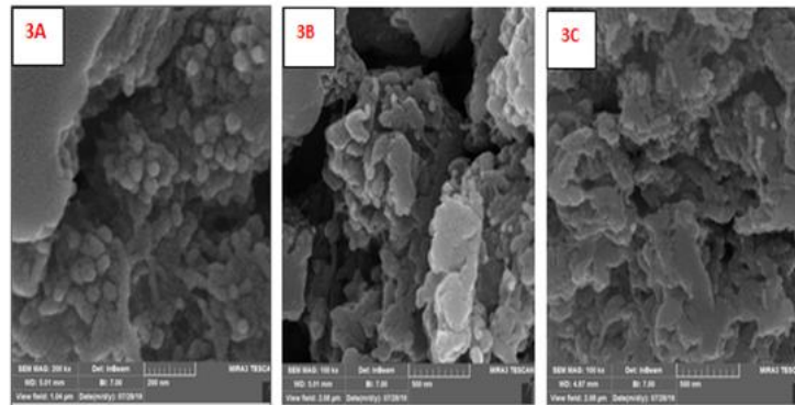
Figure 3: SEM images of the prepared PANI in (A) water, (B) 1M H_2SO_4 , and (C) 2 M H_2SO_4 .
