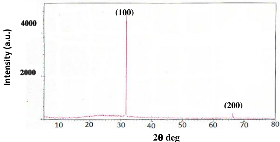
Figure 5: The XRD pattern of the CQDs sample.
