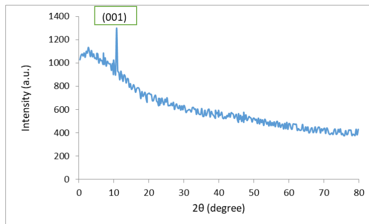
Figure 7: The XRD pattern of the CQDs/Alq 3 composite film.
