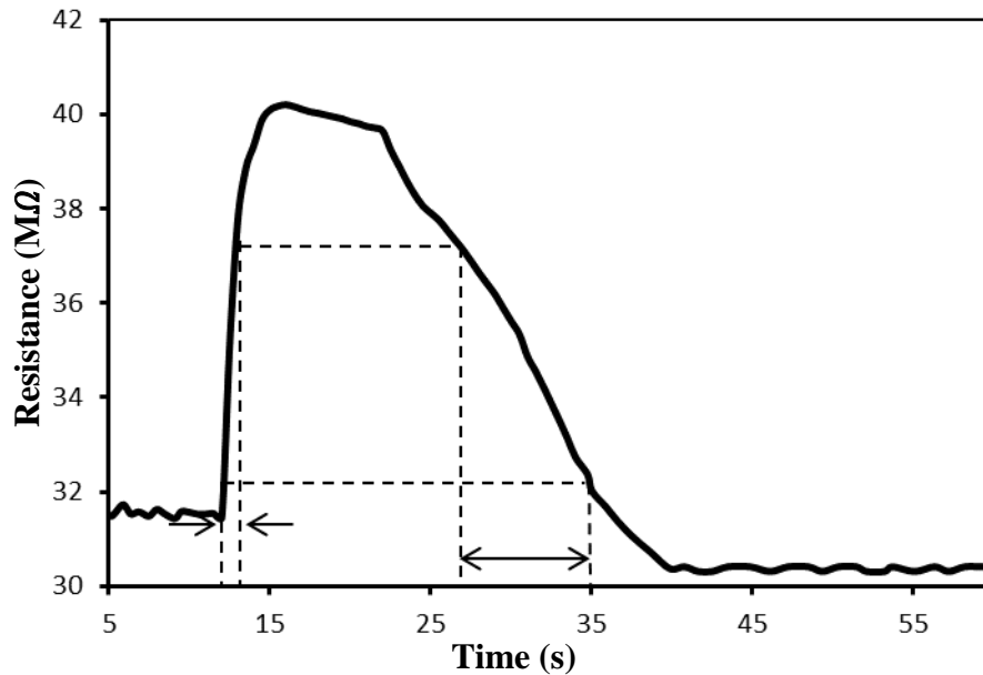
Figure 10: The resistance-time variation of CQDs/Alq 3 as a sensor to NO 2 gas at 300°C.
