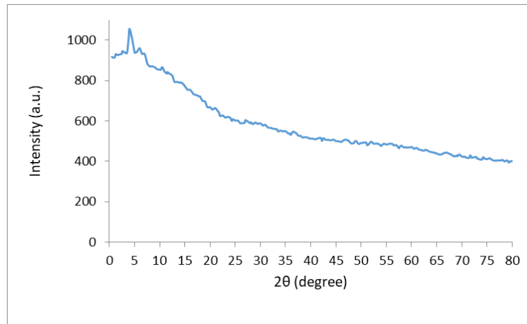
Figure 6: The XRD pattern of Alq 3 polymer.
