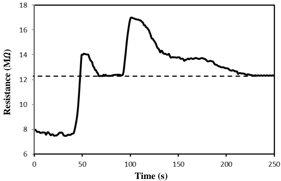
Figure 8: The resistance-time variation of \text{Alq}_3 for sensing \text{NO}_2 gas at 200^\circ\text{C} .
