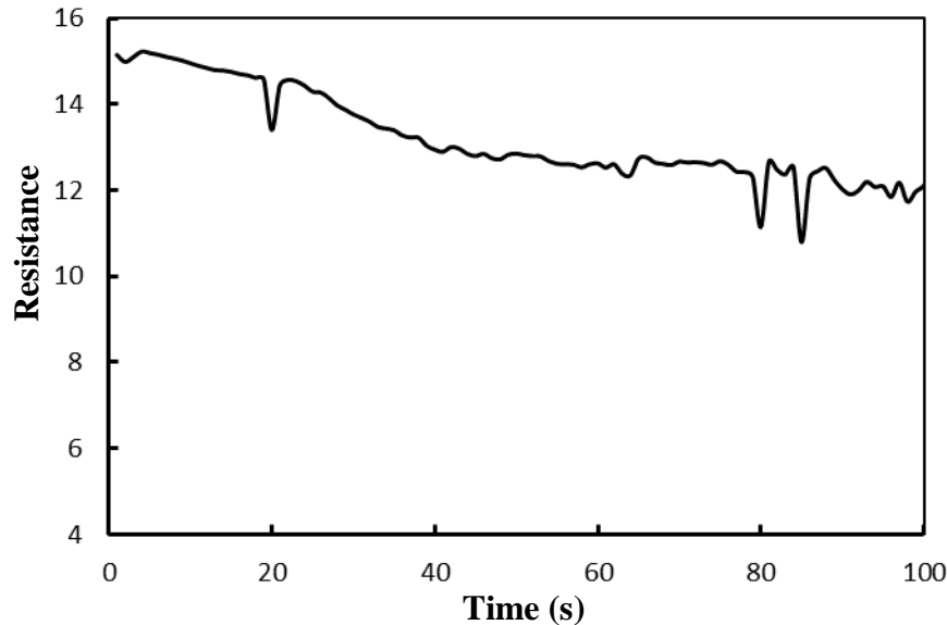
Figure 9: The resistance-time variation of Alq 3 for sensing NO 2 gas at 200°C.
